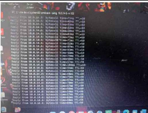
Test Ping
